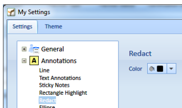
Figure 1: My Settings
